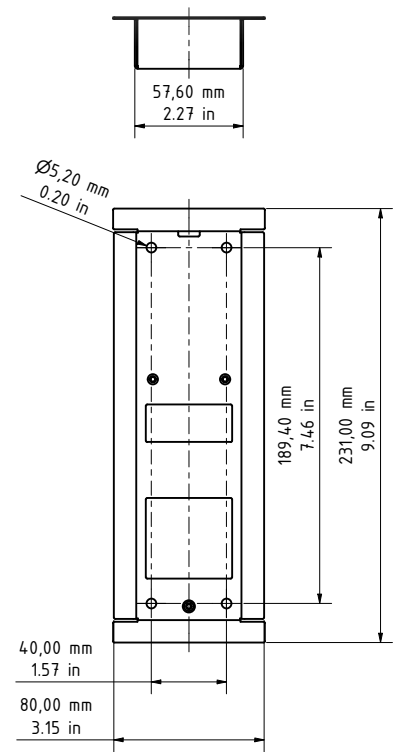
Housing (backbox)
